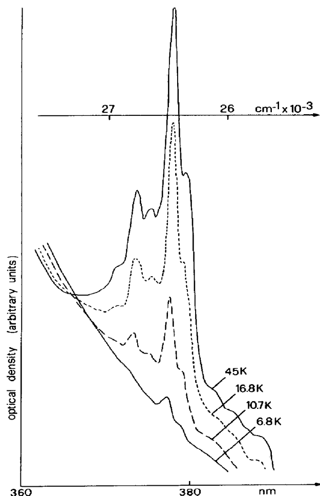
Fig. 12. Temperature dependence of the completely \vec{E} \parallel c polarized 26500 \text{ cm}^{-1} band system in vivianite, \text{Fe}_3(\text{PO}_4)_2 \cdot 8\text{H}_2\text{O} [63]. (Reprinted with permission from Inorganic Chemistry. Copyright 1983 American Chemical Society.)
