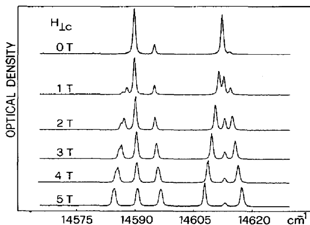
Fig. 18. Axial polarized absorption spectra of \{\text{triol}\}(\text{ClO}_4)_3 in magnetic fields ( H \perp c ) between 0 and 5 T for the lowest energy excitations at 1.5 K [4]. (Reprinted with permission from Molecular Physics.)
