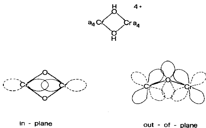
Fig. 8. Exchange interaction pathways in [a_4\text{Cr}(\text{OH})_2\text{Cra}_4]^{4+} complexes [31]. (Reprinted with permission from ACS Symposium Series. Copyright 1986 American Chemical Society.)
