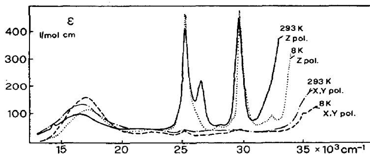
Fig. 9. Polarized crystal absorption spectra of basic rhodo perchlorate at 8 and 293 K [33]. (Reprinted with permission from Chemical Physics.)
