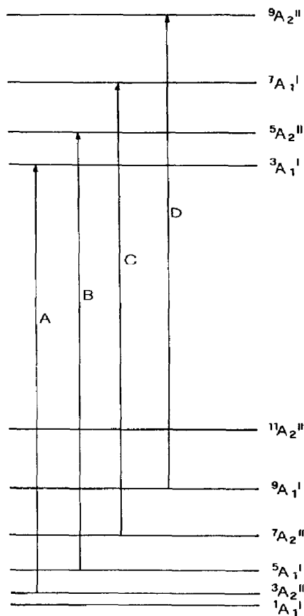
Fig. 6. Single excitations to {}^4A_1{}^6A_1 in \text{Mn}_2\text{Cl}_9^{5-} . The transitions are designated as in Fig. 4 [2]. (Reprinted with permission from Inorganic Chemistry. Copyright 1984 American Chemical Society.)
